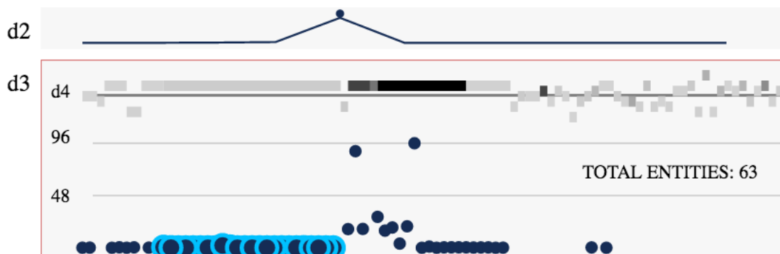
Figure 24 Expanded level 3 in detail. Circles encode nodes at level 3. Horizontal bars encode parents that contribute to the nodes directly under it.
