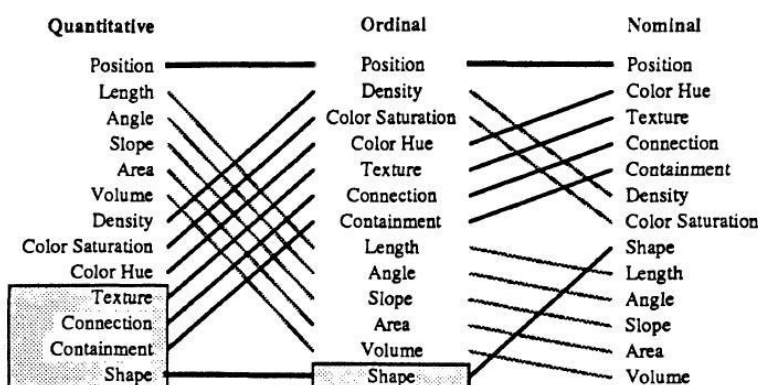
Figure 12 Appropriateness of visual variables based on data type, adapted from (Card et al., 1999)
